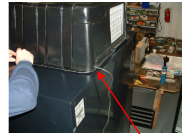
INSTALL HOLD DOWN STRAPS AND BOLTS TRAP POWER CORD UNDER STRAIN RELIEF
