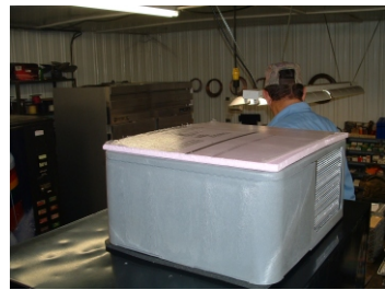
INSTALL RIGID FOAM BOARD ON TOP OF UNIT
