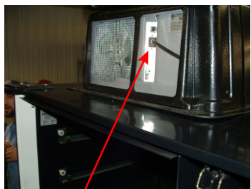
ATTACH POWER CORD TO THE UNIT AND SET THE TEMPERATURE DIP SWITCHES ( 70 DEGREES RECOMMENDED )
