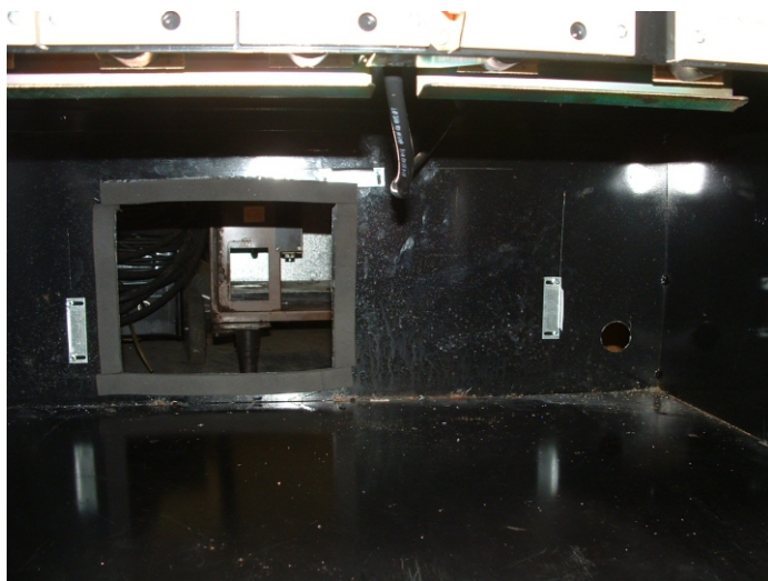
INSTALL GUIDE BRACKETS AND CABINET SEAL TO REAR WALL
