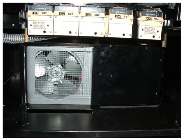
INSTALL OUTER HOUSING , CONNECT AIR SUPPLY HOSE, INSERT CUBE AND CONNECT POWER SUPPLY. INSTALL RIGHT SIDE PANEL.
