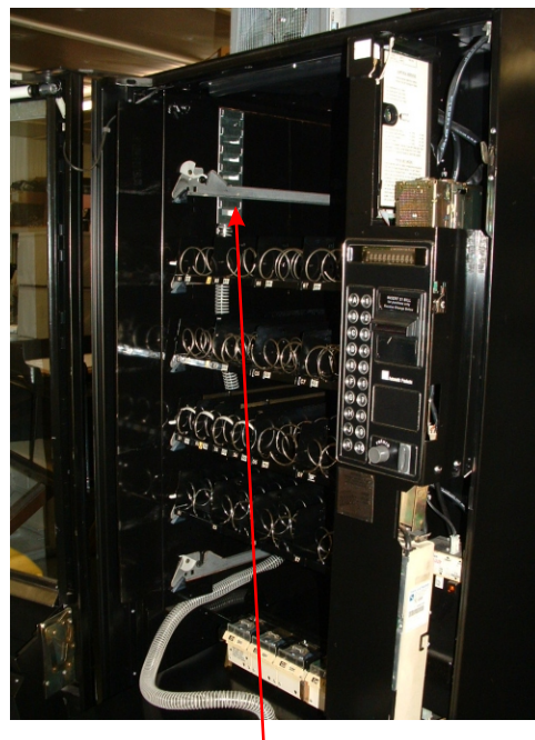
INSTALL AIR DISTRIBUTOR WITH SUPPLY HOSE FROM TOP LEFT OF CABINET.
